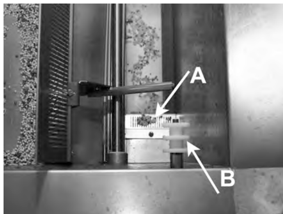
Fig. 29 Clean bottom sieve and level sensor
